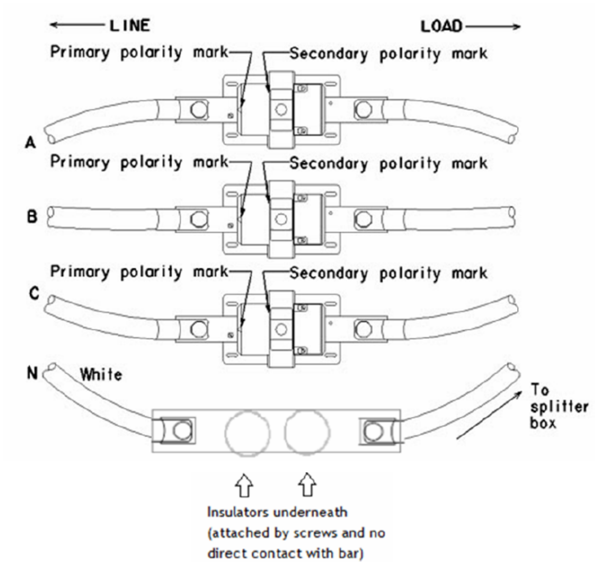
Figure 4: Three Phase CT Layout
